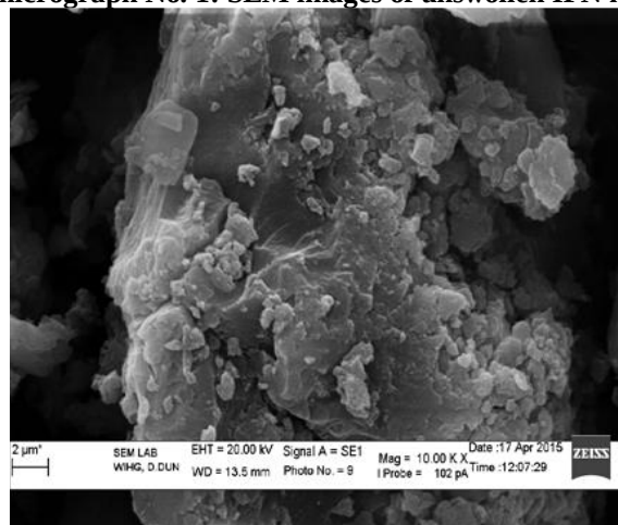
Photomicrograph No. 1: SEM images of unswollen IPN hydrogel
