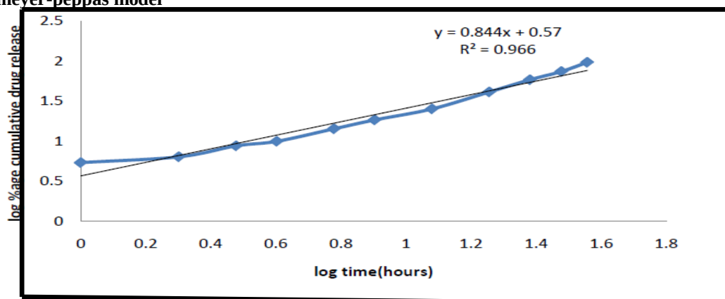
Figure No. 17: Korsmeyer-peppas model release kinetics of IPN Hydrogel formulation and Percentage cumulative drug release studies of IPN hydrogel stored at refrigeration temperature ( 4^{\circ}\text{C} \pm 2^{\circ}\text{C} ), 25^{\circ}\text{C} \pm 2^{\circ}\text{C} / 60\% \pm 5\% RH and 40^{\circ}\text{C} \pm 2^{\circ}\text{C} / 75\% \pm 5\% RH in humidity chamber.
