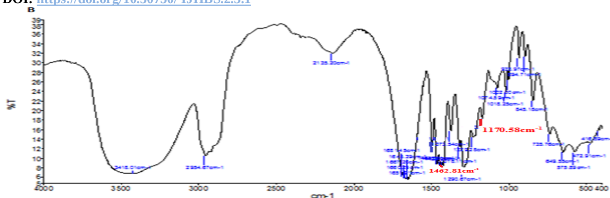
Figure No. 7:Fourier transform infrared spectrum of Poly vinyl pyrrolidone
